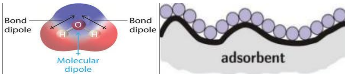
Fig. 12 Left) Polarity of an H_2O molecule. Right) Molecules adhering to the surface of an adsorbent material.
