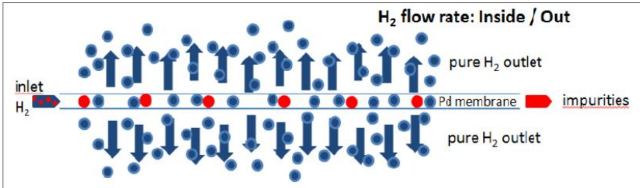
Fig. 14 Principle of operation of a Palladium membrane.
