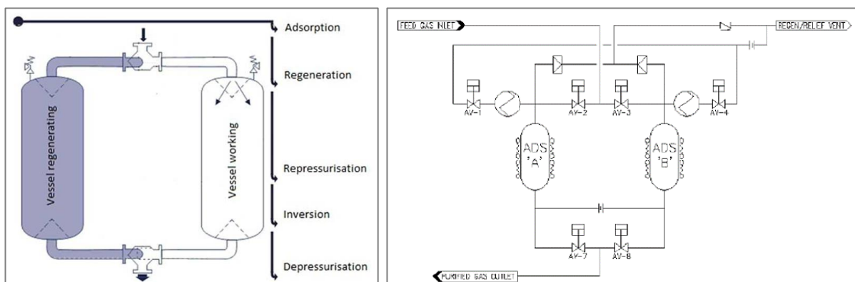
Fig. 13 PSA process block diagrams.
