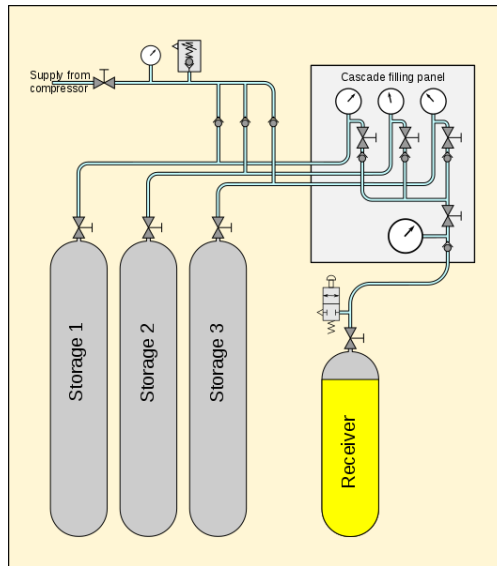
Fig. 19 Schematic diagram of a simple cascade filling system commonly used in hydrogen systems.
