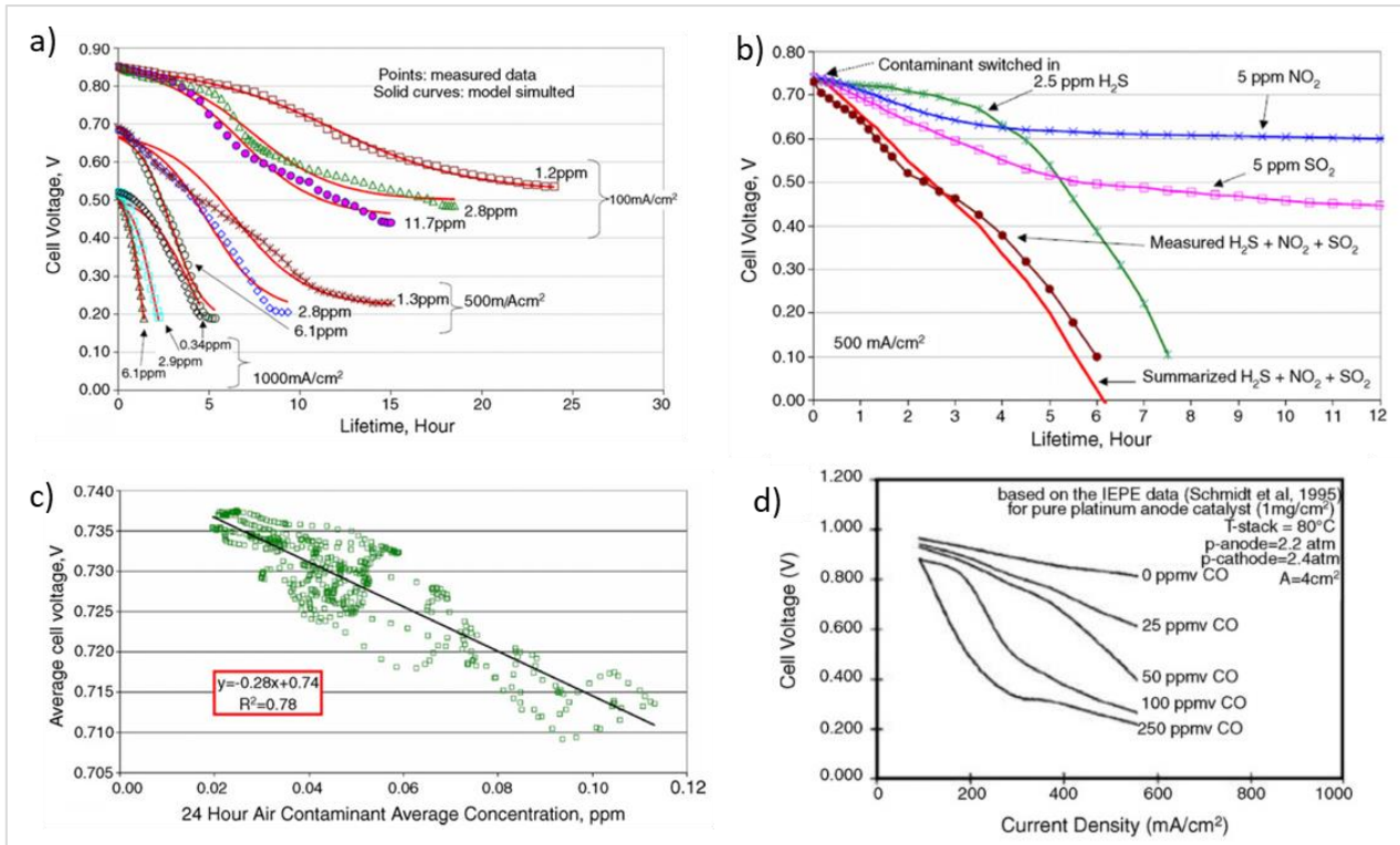
Fig. 10 a) Effect of H 2 S contamination on cell performance and lifetime. b) Individual and combined effects of 5ppm NO 2 and 5ppm SO 2 in air and 2.5ppm H 2 S in fuel on cell voltages and lifetime. c) Average cell voltage as a function of 24h average NO x concentration. d) Effects of CO concentration on cell performance. (3)
